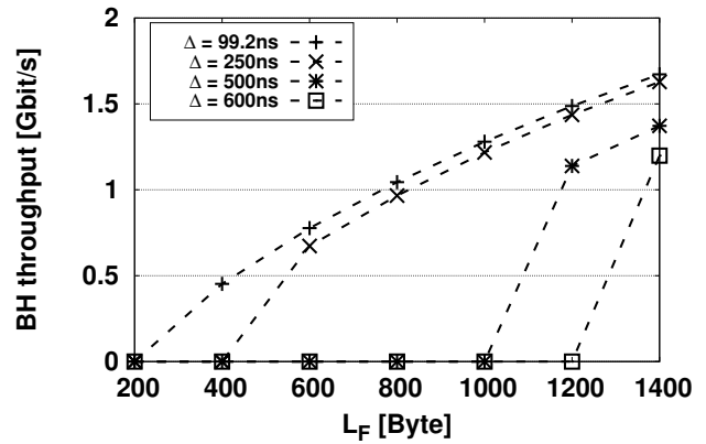
Fig. 6. BH throughput as a function of payload length L_F for CPRI opt. 6 and different \Delta when BH payloads L_B = 600 B.
